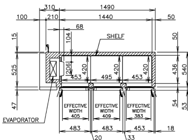
VIEW A(1/10)
