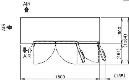
VIEW A(1/10)
