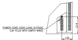
VIEW A(1/10)
